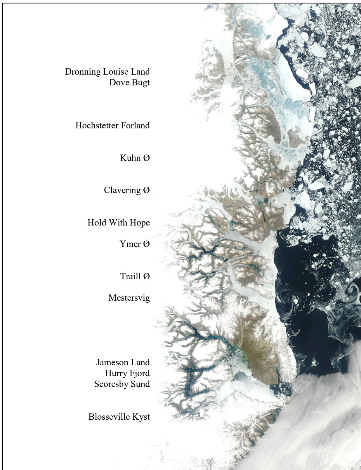
Satellite image of the Flora region on July 7 th 2009 provided by the Dundee Satellite Receiving Station. Note the early disappearance of the ice in the inner fjords and the extensive snow-free areas from Jameson Land to Hochstetter Forland.
